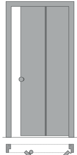
Bi-fold
